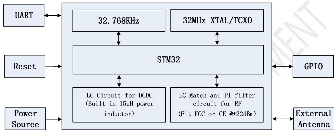
Figure 2.1: HJ-LPWE5 functional block diagram
