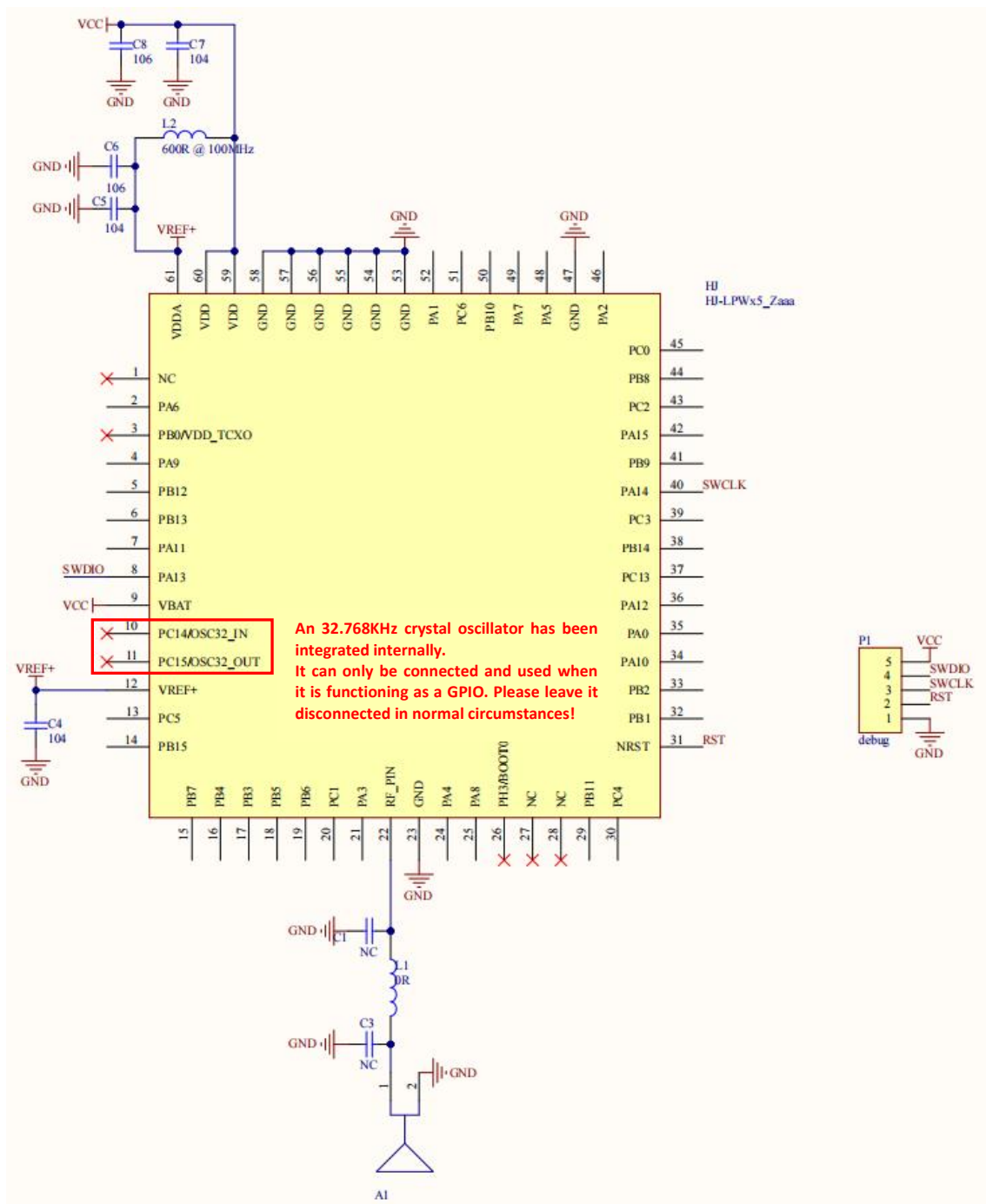
Figure 5.1: Reference schematic diagram
