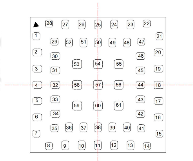
Figure 2.2: HJ-LPWE5 Pins distribution diagram
