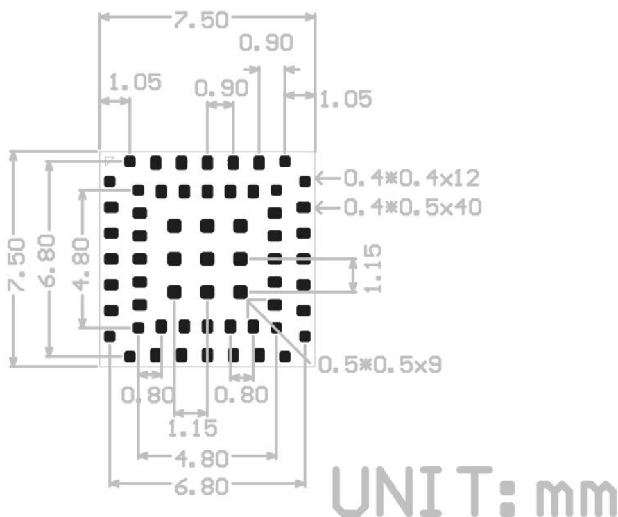
Figure 6.2: HJ-LPWE5 Package size drawing
